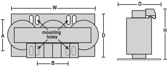
1-60 HP; 2-80 Amp
