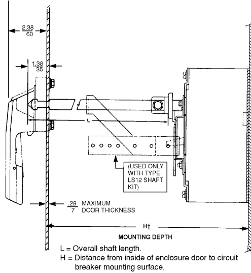
Figure 2 Side View
