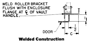
Welded Construction
