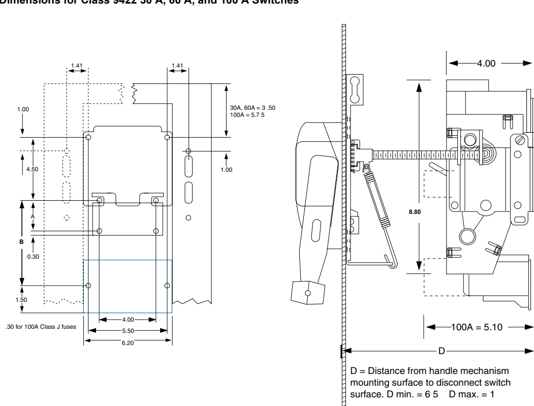
Dimensions for Class 9422 30 A, 60 A, and 100 A Switches
